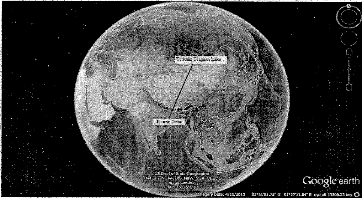
Fig:- Path of Bar-headed Goose sighted at Konar Dam, Hazaribag, Jharkhand
